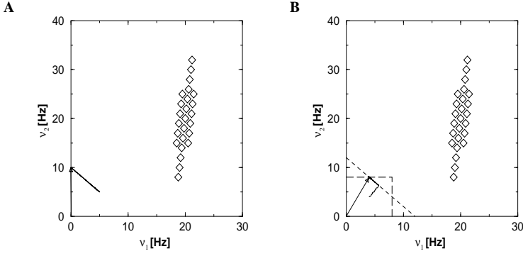
Fig. 7. Subtractive normalization in rate-based learning. A. Two presynaptic inputs with rate patterns indicated by the diamonds. The initial value of the weights is w_{i1} = w_{i2} = 5 . During learning combined with subtractive normalization as in Eq. (8.6) the rate vector moves along a line defined by the normalization condition w_{i1} + w_{i2} = \text{const} . The final position of the weight vector is indicated by an arrow. B. Three presynaptic inputs. The first two components \nu_1, \nu_2 are the same as above while the third component has a fixed rate \nu_3 = 20\text{Hz} which is the same for all patterns. The initial value of the weights is w_{i1} = w_{i2} = w_{i3} = 4 . During the first phase of learning, w_{i3} decreases to zero (not shown) while the first two components ( w_{i1}, w_{i2} ) of the weight vector move towards the cloud of data points until they hit the normalization bound w_{i1} + w_{i2} = 12 (dashed diagonal line). Weight evolution then continues along the diagonal line until one of the weights has reached its maximum value w_{\text{max}} = 8 . The final position of the weight vector ( w_{i1}, w_{i2} ) is shown by an arrow. The hard bounds w_{ij} \leq w_{\text{max}} are indicated by the long-dashed line.
