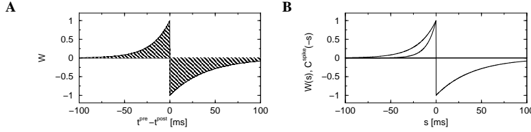
Fig. 5. STDP learning window with A_+ = -A_- = 1 and time constants \tau_+ = 20\text{ms} and \tau_- = 40\text{ms} . A. The integral over the learning window \overline{W} = \int W(s) ds is negative so that \alpha = -\overline{W} > 0 . B. The parameter \beta is defined by the overlap between the window function (thin line) and the spike correlations, \beta = \int W(s) C^{\text{spike}}(-s) ds . Here we assumed a time constant \tau_C = 10\text{ms} for C^{\text{spike}} .
