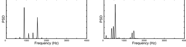
Fig. 2. Example of spectral GMM states for female [left] and male [right] speakers. Each state i is represented by its PSD : r_i^2(f) .
