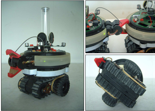
Fig. 1. Left: The s-bot . Above Right: The s-bot connection mechanism. Below Right: The s-bot traction system.
