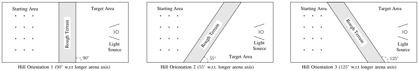
Fig. 2. Scale diagram of the three possible hill orientations. The arena for each of the seven environments used in this study measures 210 cm x 105 cm. Three environments contain the ‘moderate’ hill (2.8 cm high, navigable by a single s-bot ). Three environments contain the ‘difficult’ hill (6.5 cm high, not navigable by a single s-bot ). One environment has no hill. The starting area and target area are demarcated by the hill and the arena boundaries (in the no-hill environment the target area is considered to be the same as for environments with hill orientation 1). Starting positions are marked by crosses.
