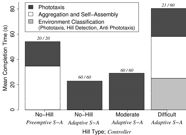
Fig. 5. Break-down of mean completion times for s-bots using the preemptive self-assembly controller (left bar) and the adaptive self-assembly controller (right three bars) in no-hill, moderate hill and difficult hill environments. Only data from completed trials are presented (number of completed trials and number of trials in total are indicated above each bar).
