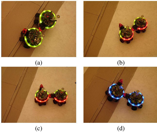
Fig. 7. Execution of the morphology aware controller. (a): The s-bots have already adaptively aggregated and self-assembled. The connected swarm-bot approaches the hill with an inappropriate orientation. (b): The swarm-bot performs antiphototaxis away from the hill and starts to rotate. (c): The swarm-bot rotates until it has a more appropriate orientation (based on memory of the hill orientation). (d): The swarm-bot recognises that it has an appropriate orientation and overcomes the hill.
