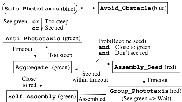
Fig. 3. Finite State Machine representing the Adaptive Self-Assembly Controller. The starting state is Solo_Phototaxis. Colours in parentheses refer to the LEDs that are illuminated in the corresponding state.
