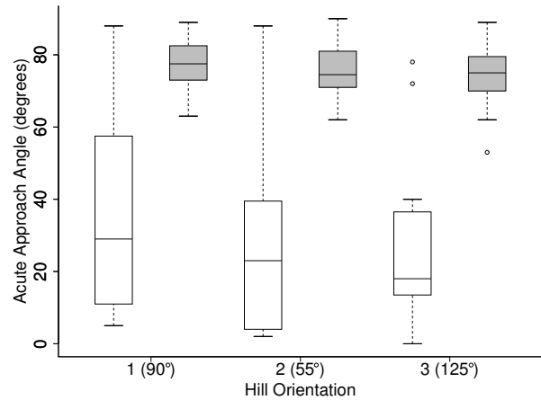
Fig. 8. Box-and-whisker plot showing acute approach angles (orientation of the swarm-bot with respect to the orientation of the hill when the swarm-bot first makes contact with the hill). If the swarm-bot approached the hill more than once, only data from the final approach is shown. Each box represents 20 trials. White boxes: swarm-bots without morphology awareness. Gray boxes: swarm-bots with morphology awareness.
