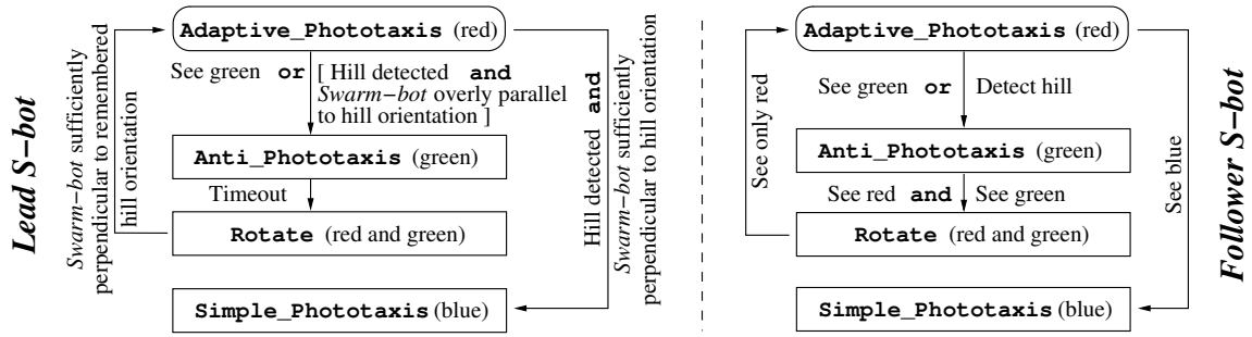
Fig. 6. The morphology aware controller — finite state machine extension of the adaptive self-assembly controller. The s-bot first executes the adaptive self-assembly controller (see Fig. 3). However, instead of executing the Group_Phototaxis state the s-bot switches into state Adaptive_Phototaxis , either as a lead s-bot (the s-bot that seeded self-assembly) or as a follower s-bot (all other s-bots ).
