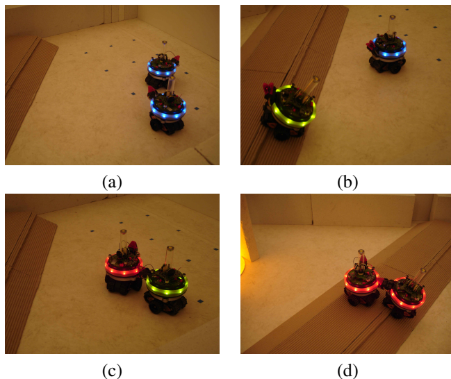
Fig. 4. (a): Two s-bots start from random positions and orientations. Initially, they perform individual phototaxis, and have their blue LEDs illuminated. (b): One s-bot detects a slope it cannot overcome alone and illuminates green LEDs. The other s-bot detects colour green (local communication). (c): The group aggregates and self-assembles. (d): The s-bots collectively overcome the rough terrain and reach the target area
