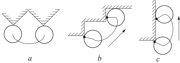
Fig. 9. Worst cases. (a): not losing contact, (b): not slipping, (c): maximal wheel actuator torque
