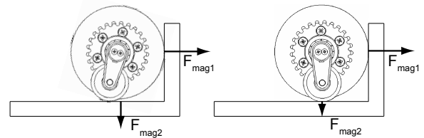
Fig. 3. The lever arm mechanism is applied, in order to slightly lift off the wheel and locally decrease the unwanted magnetic force F_{mag2} [6]
