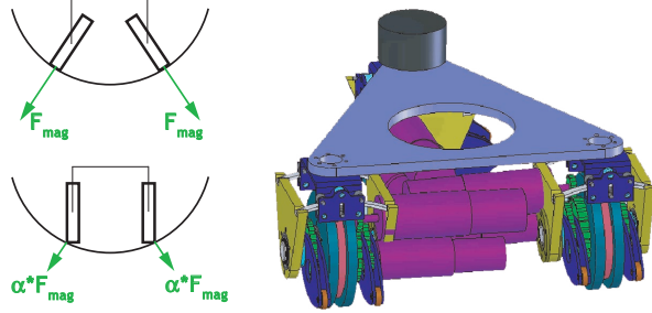
Fig. 5. Left: magnetic wheel without and with ground adaptation. Right: example of a 3 magnetic wheels robot with cumbersome passive mechanics and actuators
